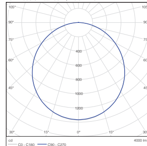
LED Panel Delta Pro 40W 4000K 60x60
