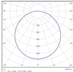
LED Panel Delta Pro 40W 3000K 60x60
