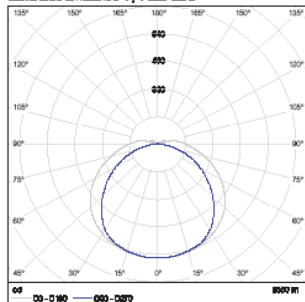
TL Waterproof Poseidon 33W 4000K 1580mm
